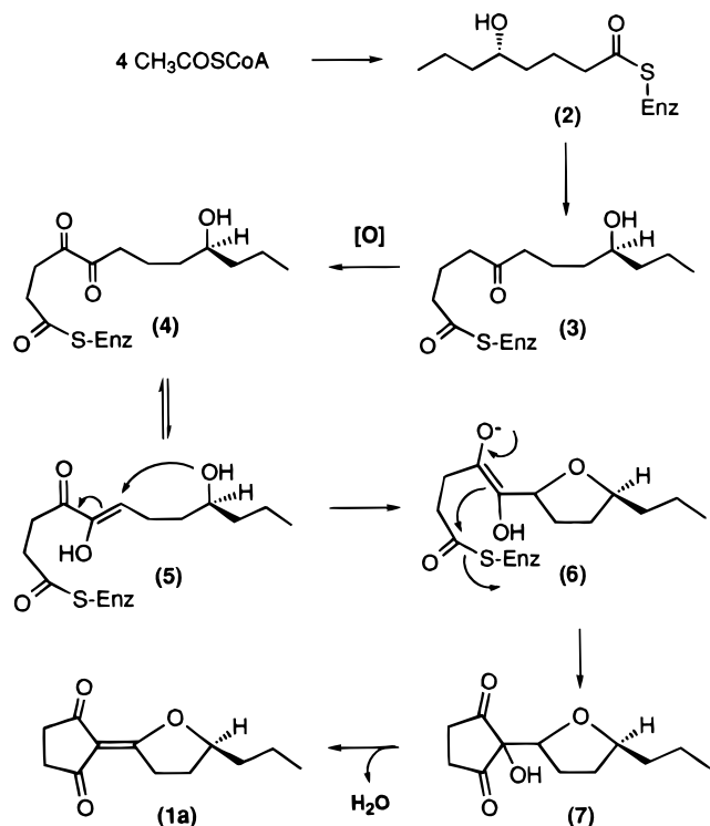
Scheme 2. Plausible Mechanisms for the Biogenesis of Oudenone (1a)
