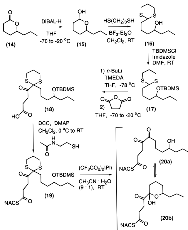
Scheme 3. Synthesis of \alpha -Diketone NAC Thioester 23
